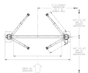
Fig 1b - Service Bay Layout
